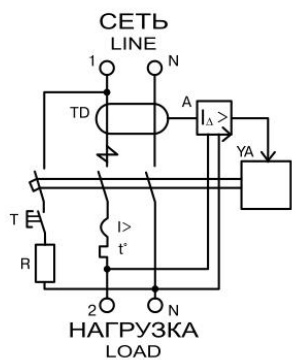
АВДТ32 (In 6-40 A)
