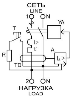
АВДТ32 (In 50 A, 63 A)
